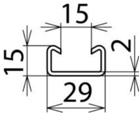
Dimension drawing AK SAK 1000 V2A
