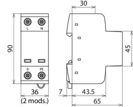
Dimension drawing DSH TN 255
