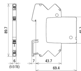
Dimension drawing BCO ML2 BE 180
