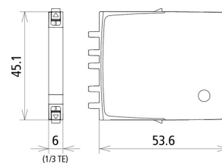
Dimension drawing BCO MOD ML2 BD 180
