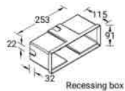
Recessing box
