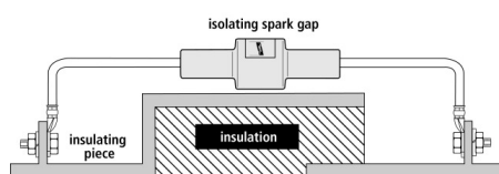
Installation of EXFS 100 KU
