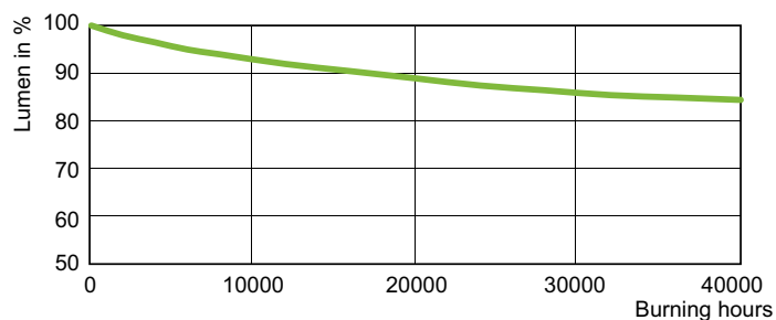
LDLM_SONTAPIA_0004-Lumen maintenance diagram
