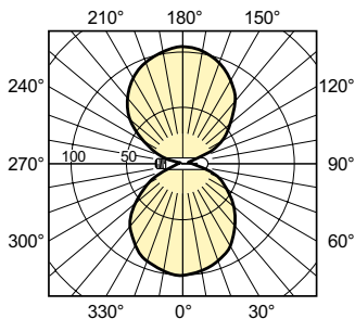
LDLD_SONTAPIA-Light distribution diagram
