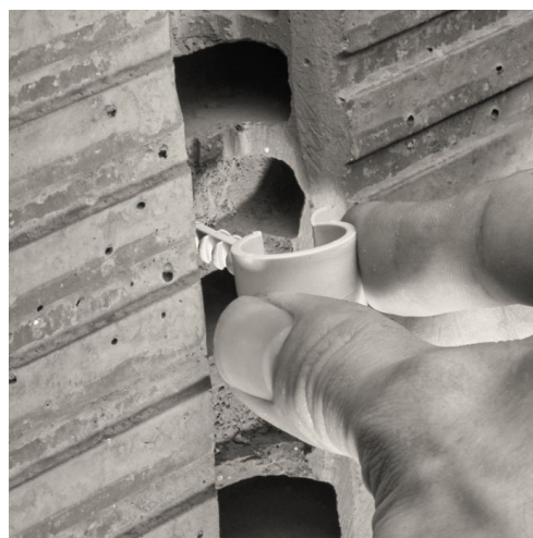
Simply brilliant: the integrated nib on the interior side of the clip enables the pipe to tense between the two clips for easier cable insertion.
