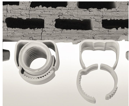
An innovative product for sub-plaster mounting - the Buried Clamp Automatic USA. A quick push is enough to affix the clamp to the pipe.
