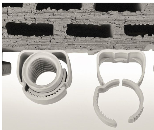
An innovative product for sub-plaster mounting - the Buried Clamp Automatic USA. A quick push is enough to affix the clamp to the pipe.
