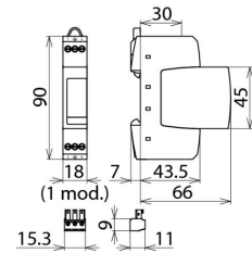
Dimension drawing DR M 2P 30 FM
