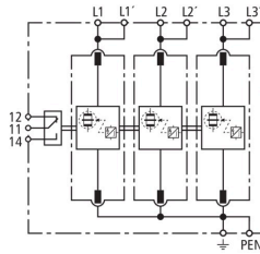
Basic circuit diagram DV M TNC 255 FM
