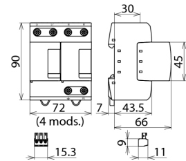
Dimension drawing DV M TT 2P 255 FM
