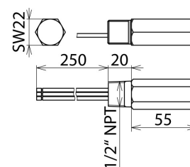
Dimension drawing DPI CD EXD 24 N
