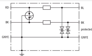
Basic circuit diagram DPI ME 24 N A2G
