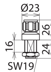
Dimension drawing DGA G N
