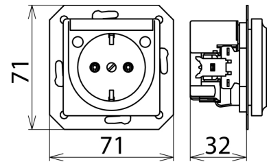
Dimension drawing NSM PRO TW
