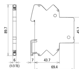
Dimension drawing BCO CL2 BD 12
