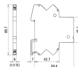
Dimension drawing BCO CL2 BE 48
