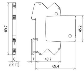
Dimension drawing BCO ML2 BE 48
