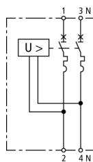
Basic circuit diagram POP 2 255 C40
