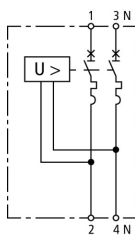
Basic circuit diagram POP 2 255 C25
