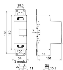
Dimension drawing DBM 1 CI 760 FM
