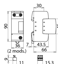
Dimension drawing DGP M 255 FM
