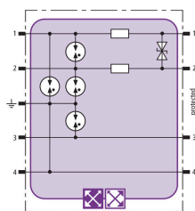
Basic circuit diagram BXT ML2 BD S EX 24
