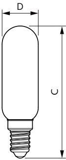
Bulb T25 230V 3-25W 250lm2700K E14 ND CL
