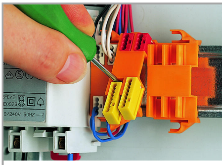
Removing a mounting carrier from the assembly.
