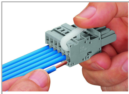
Operating lever
