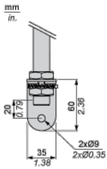
Dimensions for Metal Bracket
