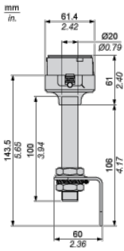
Dimensions for Metal Bracket
