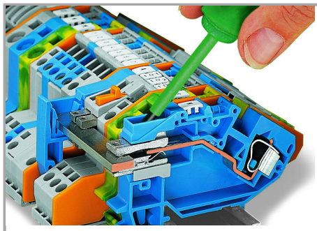
Operating an N-disconnect slide link.
