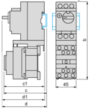
Combination GV2P + TeSys d contactor
