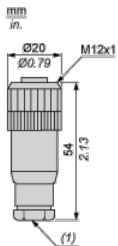
(1) Cable gland : no. 7 plastic (Pg 7)
