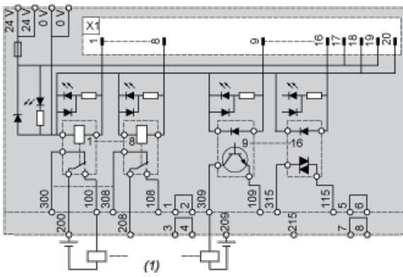
(1) 16 channels
