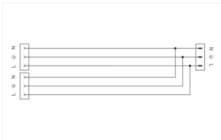
Cable assembly WINSTA ® RD with strain relief
