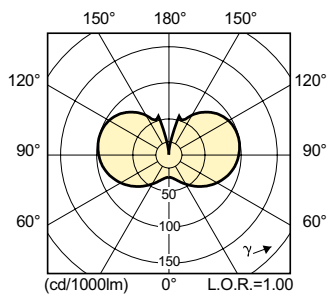
LDLD_CDO-TT_0006-Light distribution diagram
