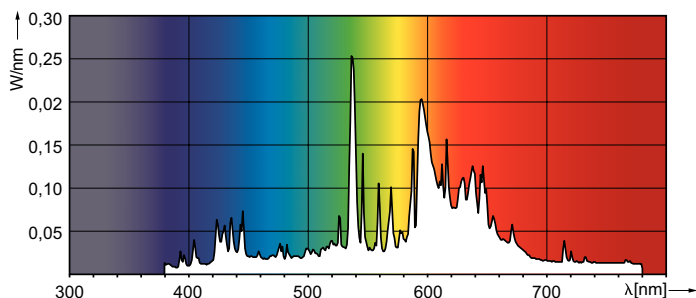
LDPO_CDO-TT_0001-Spectral power distribution Colour
