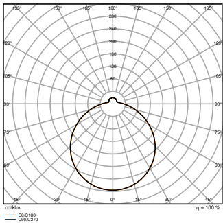
SF CIRC 500 V 42W 840 IP44 PS 2500lm
