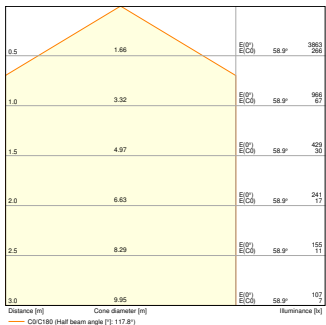
SF CIRC 500 V 42W 840 IP44 PS 3500lm
