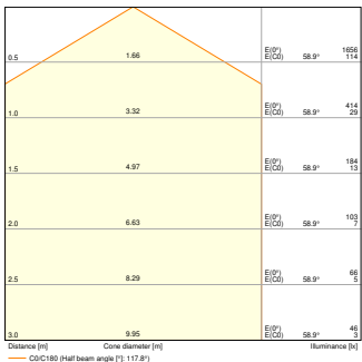
SF CIRC 500 V 42W 840 IP44 PS 1500lm
