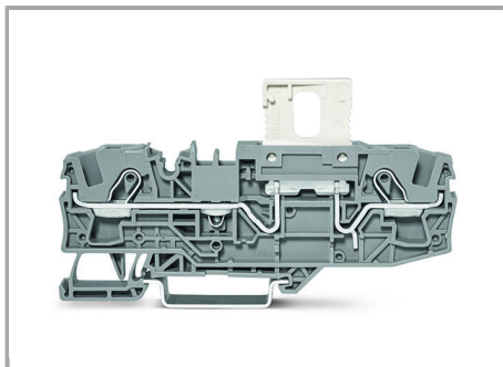
Carrier terminal block (2006-401/050-000) with disconnect plug (2006-1661) in operating position
