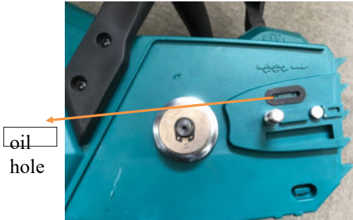
Use a slotted screwdriver to clean the oil hole
