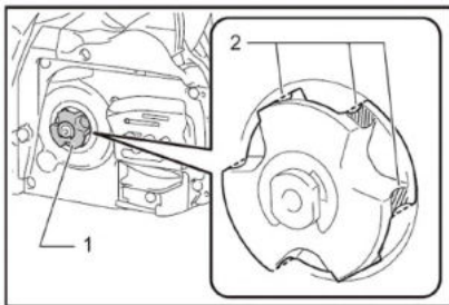
Use a slotted screwdriver to clean the oil hole
