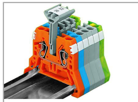
In addition to the plastic marker strips, group marker carriers are now available for the WMB and WSB marking systems. They can be mounted parallel to a push-in type jumper bar via open jumper contact slot. It assists with viewing marker slots on the side of the terminal block. Group marker carriers are available in 5 mm/0.197 inch, 10 mm/0.394 inch and 15 mm/0.591 inch widths.
