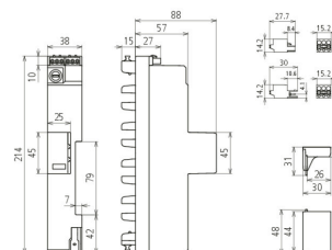
Dimension drawing DSH ZP 2 SG TNS 255
