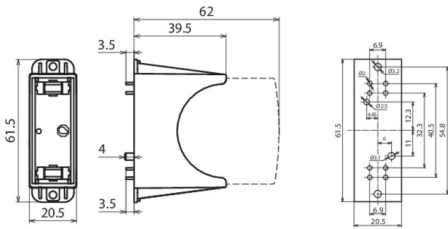
Dimension drawing DG PCB PV 30
