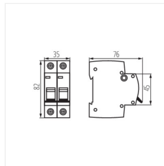
KMB6-B50/2
