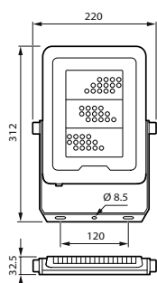
BVP164 LED73/840 PSU 70W AWB CE
