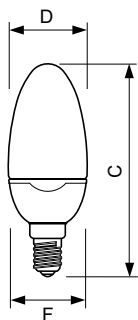
Candle 12W/827 E14 220-240V 50/60Hz
