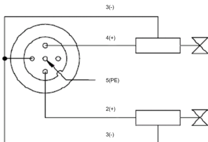
IEC Wiring Diagram with 2 Actuators
