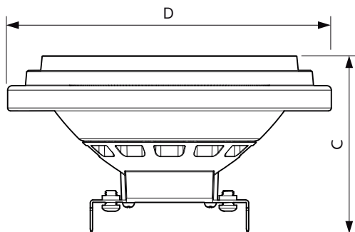
AR111 12V 11-50W 650lm 8D 3000K G53 D
