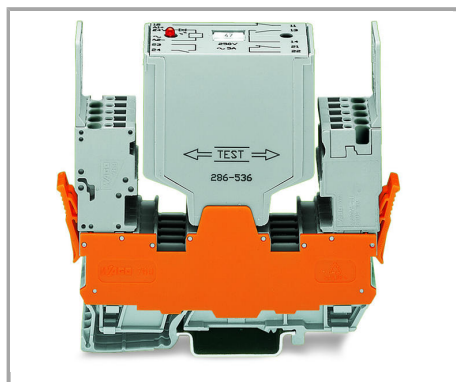
2-pin carrier terminal block for pluggable modules with orange separator plate
