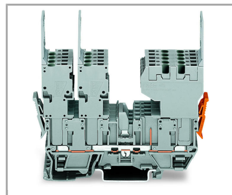
2 x 1-conductor female plug (left), 1 x 2-conductor female plug (right), may be reversed – carrier terminal blocks can be commoned via 280 and 780 Series Jumpers and tested using a 280 Series Test Plug Adapter.
