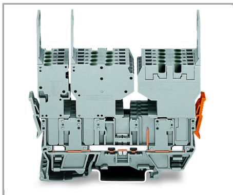
4-pin carrier terminal block
