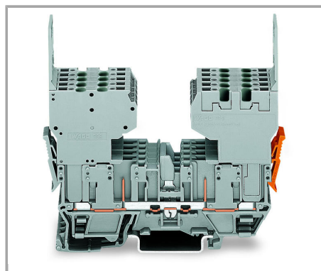
2 x 2-conductor female plugs
