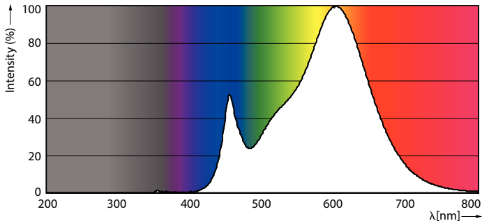
LEDcapsule 2W G9 830
