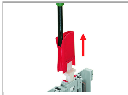
Removing a disconnect lock.
